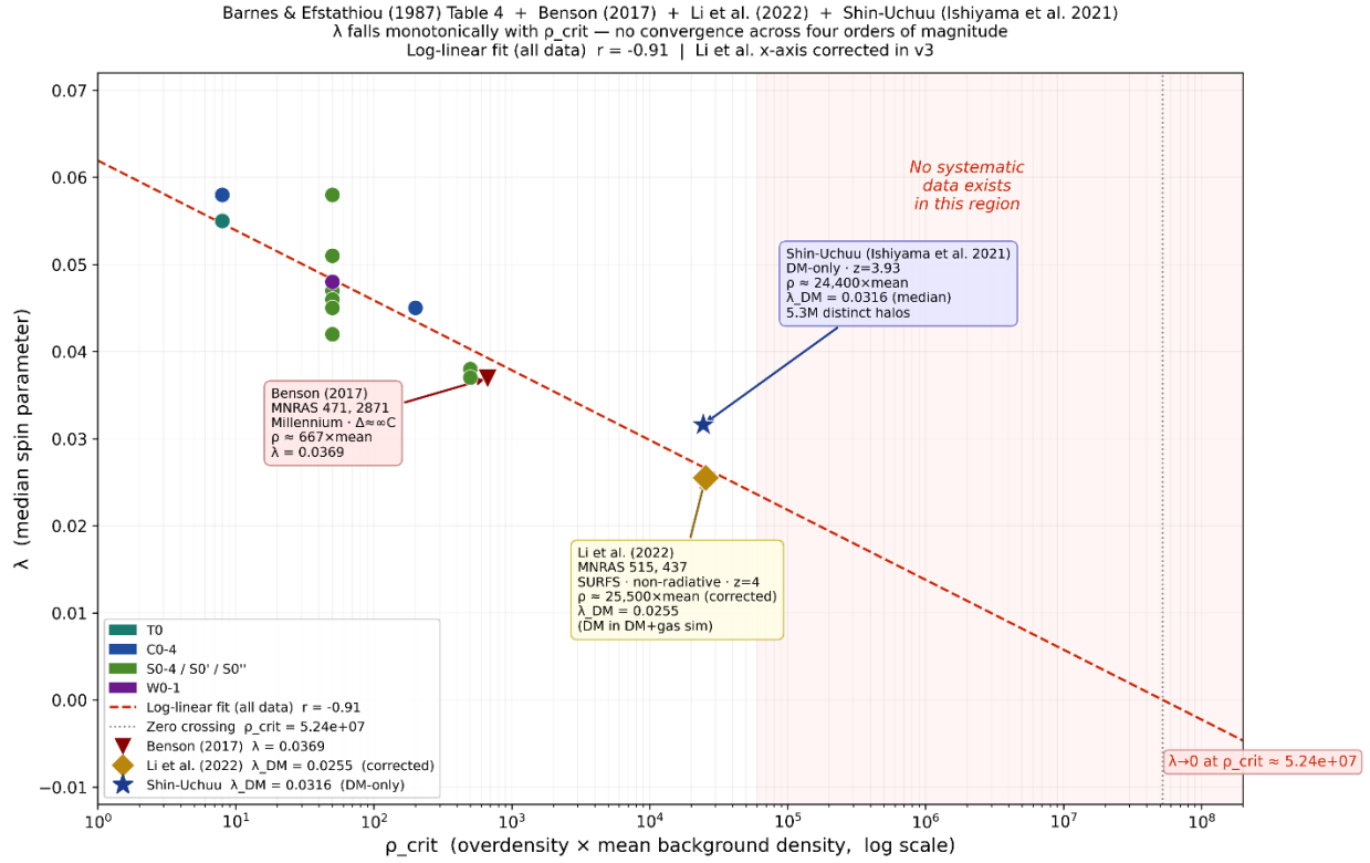
Figure 4 (revised). Halo spin parameter \lambda vs overdensity threshold p_{\text{crit}} . Barnes & Efstathiou (1987). Benson (2017), Li et al. (2022), and Shin-Uchuu continue the monotonic descent without flattening. Li et al. x-axis corrected in v3 to p_{\text{crit}} \approx 25,500 \times mean at z=0 . Dashed extrapolation projects to \lambda \rightarrow 0 at p_{\text{crit}} \approx 5.24 \times 10^7 . No free parameters in the placement of the modern points. This is the empirical measurement of E[\lambda] \rightarrow 0 predicted by A.4–A.6.
